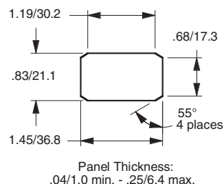
Mounting Hole
