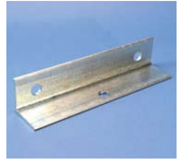
Multi-Attachment CSBMA (Imperial, Metric)
