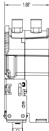
e2XHD MTP-MTP Fiber Cassette (3x8-fiber to 2x12-fiber)
