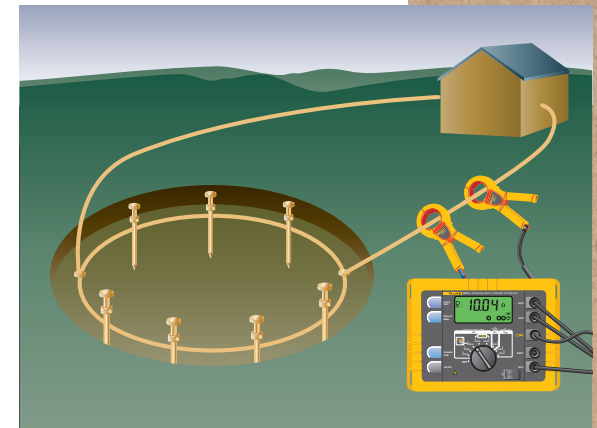
Using Stakeless testing at a remote switching site.
