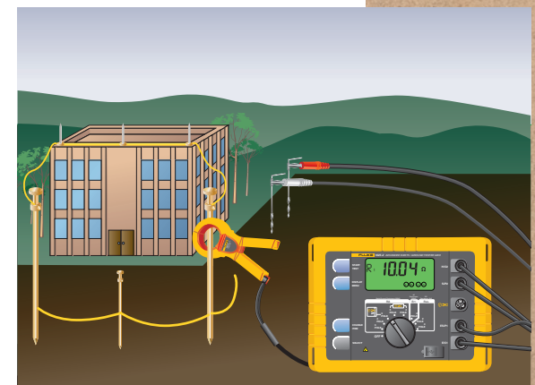
Using Selective testing on a lightning protection system.
