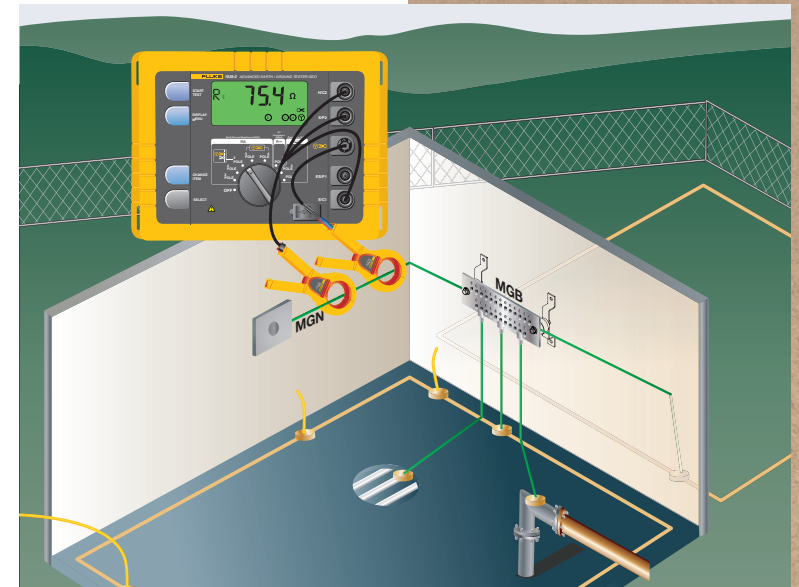
Figure 1: Stakeless testing of a central office.
