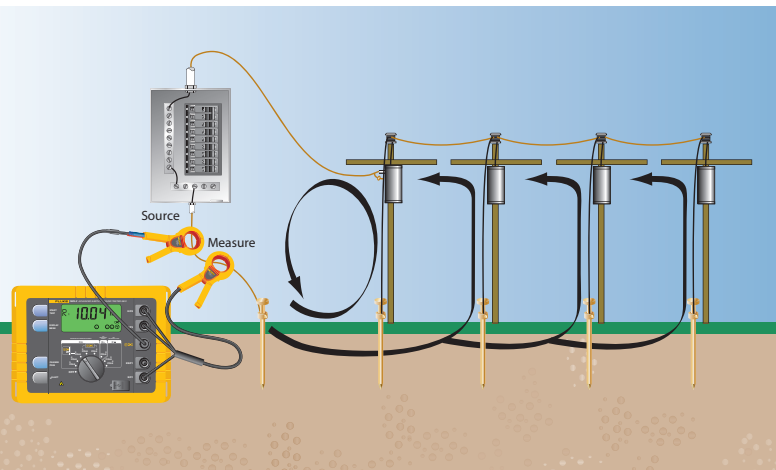
Test current paths in the stakeless method.
